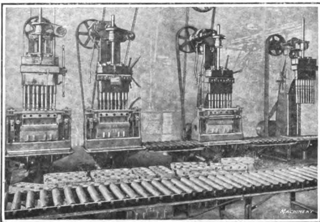
Fig. 18—Sometimes it is feasible to design jigs and fixtures in which work may be held for the performance of a number of machining operations. This illustration shows such jigs in use in the Maxwell Motor Co.'s shops in Detroit, Mich. The work and jig are pushed along from machine to machine on a roller conveyor, the operator following the jig right down the line of machines.
